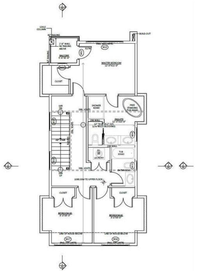
1 UPPER FLOOR PLAN A4 1/4" x 1/4" = 1'-0" LEGAL DESCRIPTION: LOT 22 BLOCK 9, MUNICIPAL ADDRESS: 254 HUNTINGTON ROAD NE
